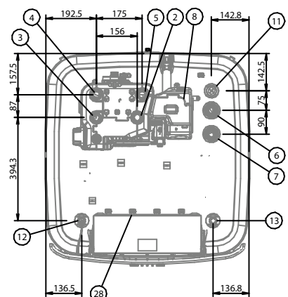
Anschlüsse
