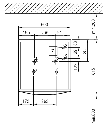
Grundriss WPNS 060–080
