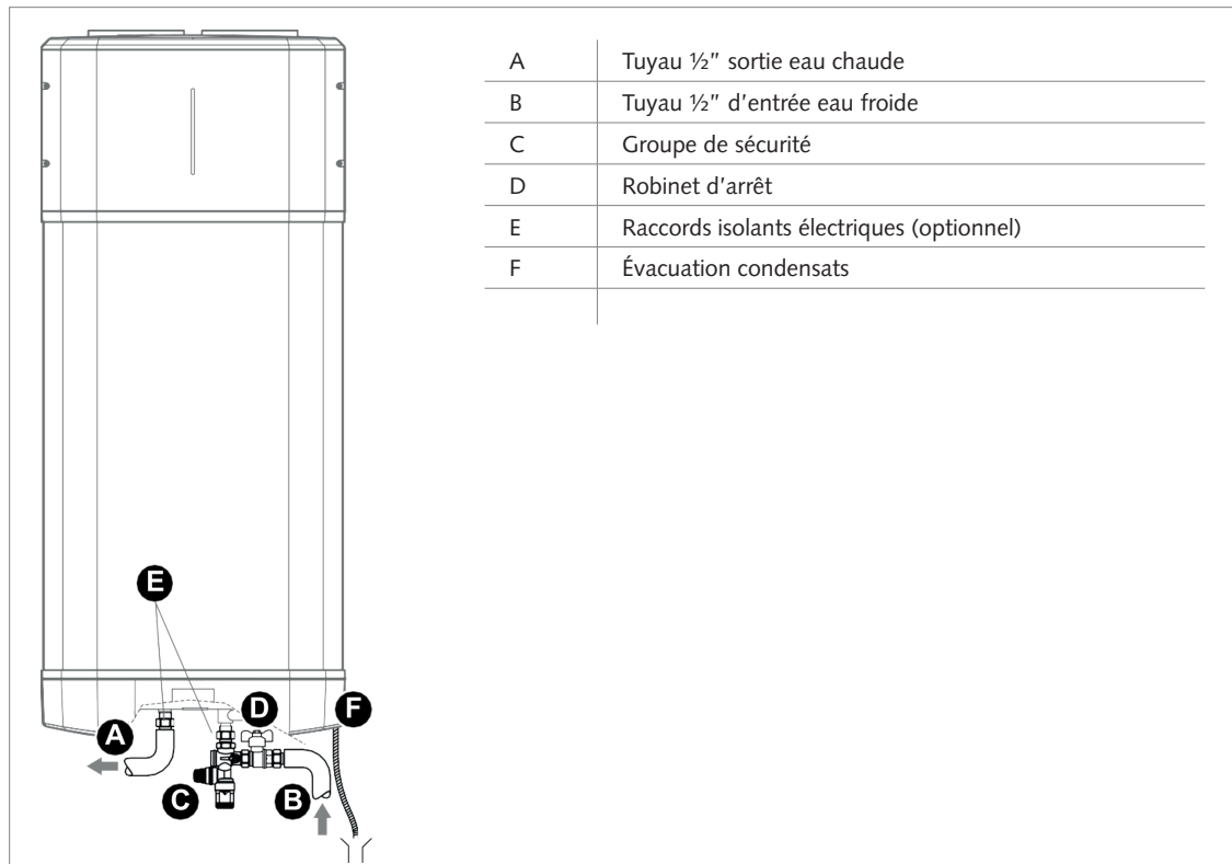
III. : Raccordements hydrauliques
